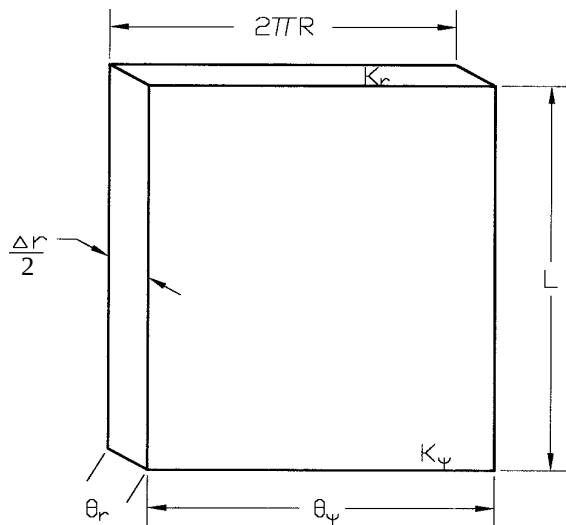
Fig. 3. Angular contribution to the radial thermal conductivity of an arbitrary turn at radial location R .
