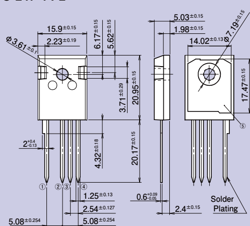
TO-247-4-P2
