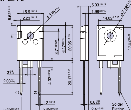
TO-247-2L-P2
