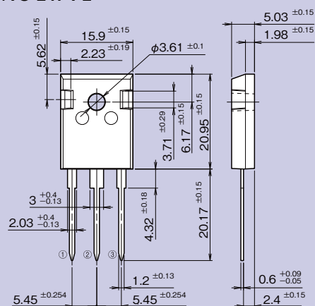
TO-247-P/TO-247-P2
