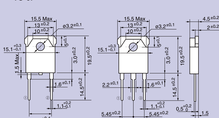
TO-3P
