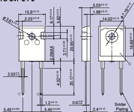
TO-247-2-P2
