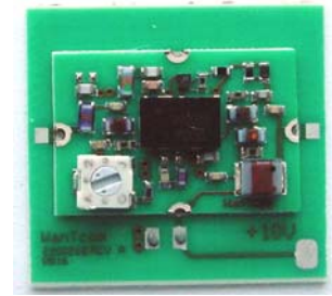
Fig. 3 Assembled part
