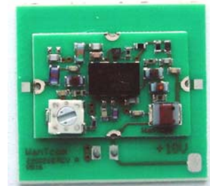
Fig. 3 Assembled part
