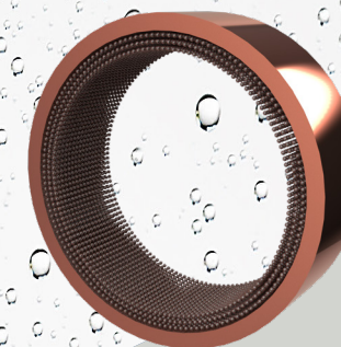
Powder Wick Heat Pipe
